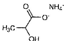
Chemical Structure of Ammonium Lactate
